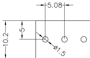
Recommended P.C.B Layout(Top Side)
