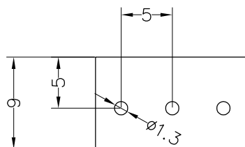
Recommended P.C.B Layout(Top Side)
