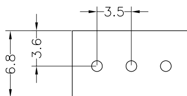
Recommended P.C.B Layout(Top Side)
