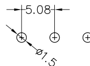
Recommended P.C.B Layout(Top Side)
